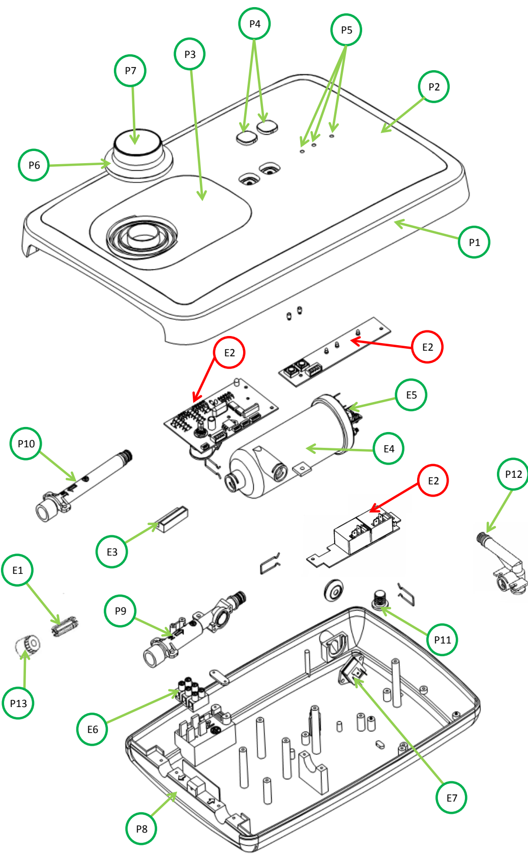
ACCESSORIES SET (B-49-L42) EWE
